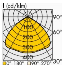
HB-E-260 – 110°
