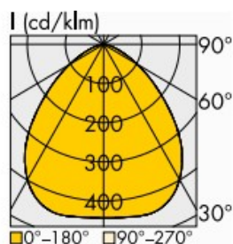
HB-E-260 – 90°
