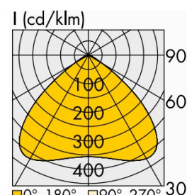
HB-E-305 – 110°
