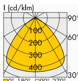
HB-E-305 – 90°
